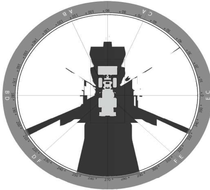
< Top view of the machine at ground level visibility without the use of optional visual aids >
